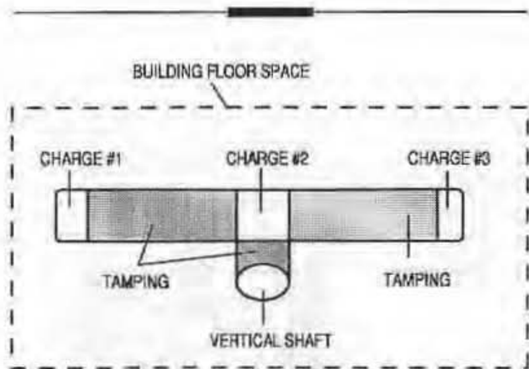
Coyote tunnel (not to scale—exaggerated for clarity).
