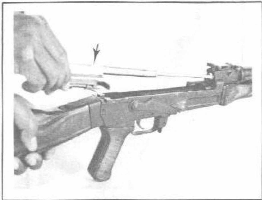
FIGURE 28. REMOVING CARRIER
