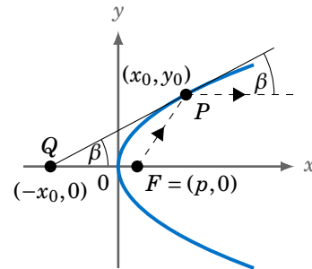
Figure 7.2.4 4px = y^2
