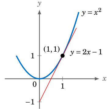
Figure 3.1.2
