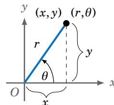
Figure 7.7.5
