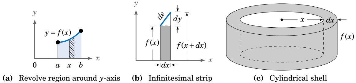
Figure 8.4.5 Shell method
