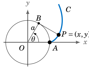
Figure 7.6.7 Exercise 8
