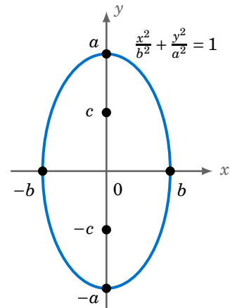
Figure 7.1.9
