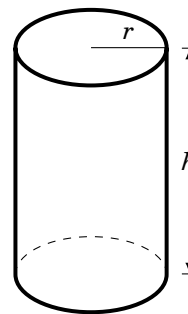
Figure 4.1.2
