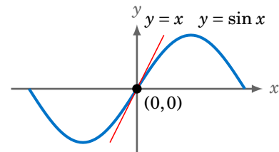
Figure 3.1.4
