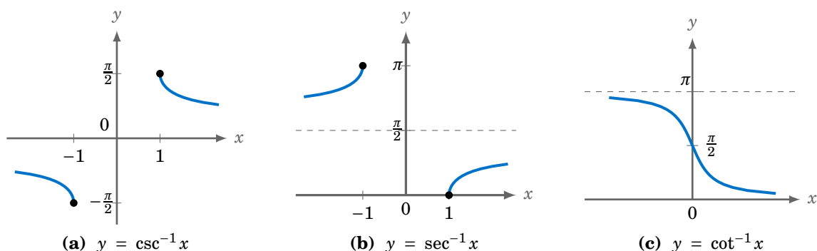
Figure 2.2.4 Graphs of \csc^{-1}x , \sec^{-1}x , \cot^{-1}x
