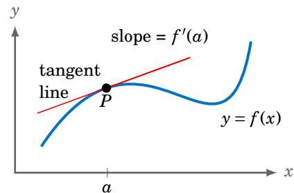
Figure 3.1.1 Tangent line
