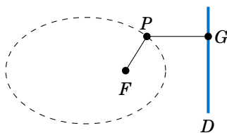
Figure 7.1.11 Exercise 13
