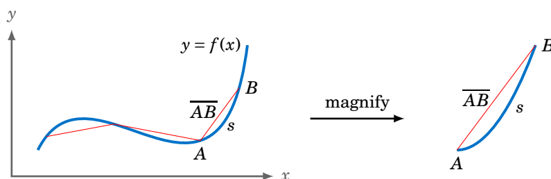
Figure 1.3.1 Curved real-valued distance s \neq length of \overline{AB} , but infinitesimal s = length of \overline{AB}
