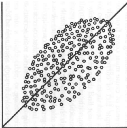
low correlation
