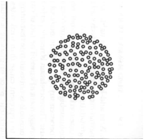
no correlation
