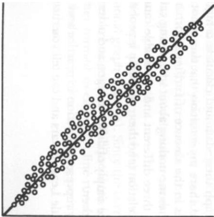
high correlation
