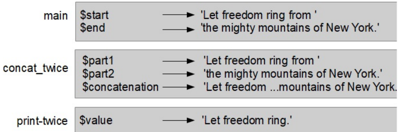
Figure 3-1. Stack diagram
