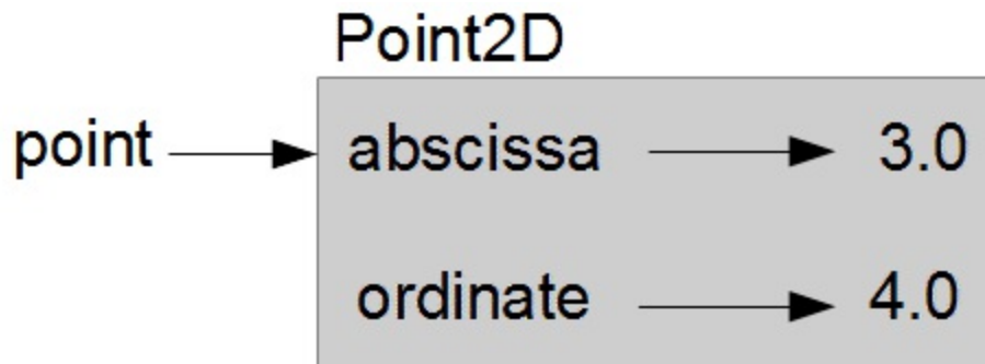
Figure 12-1. Object diagram
