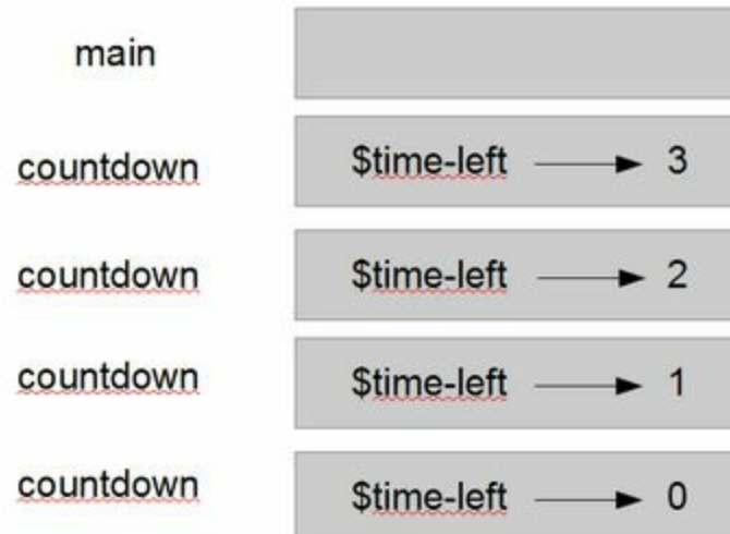
Figure 4-1. Stack diagram
