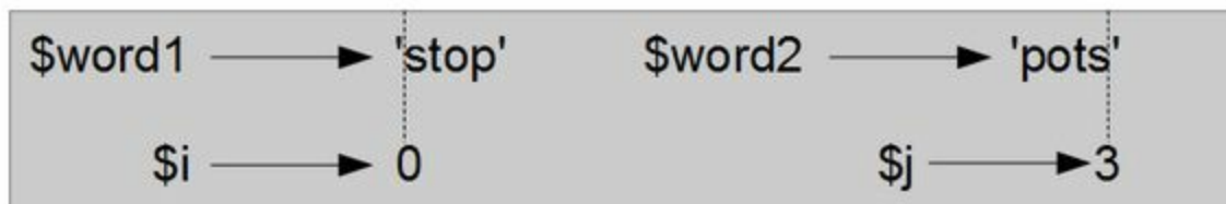
Figure 7-1. State diagram
