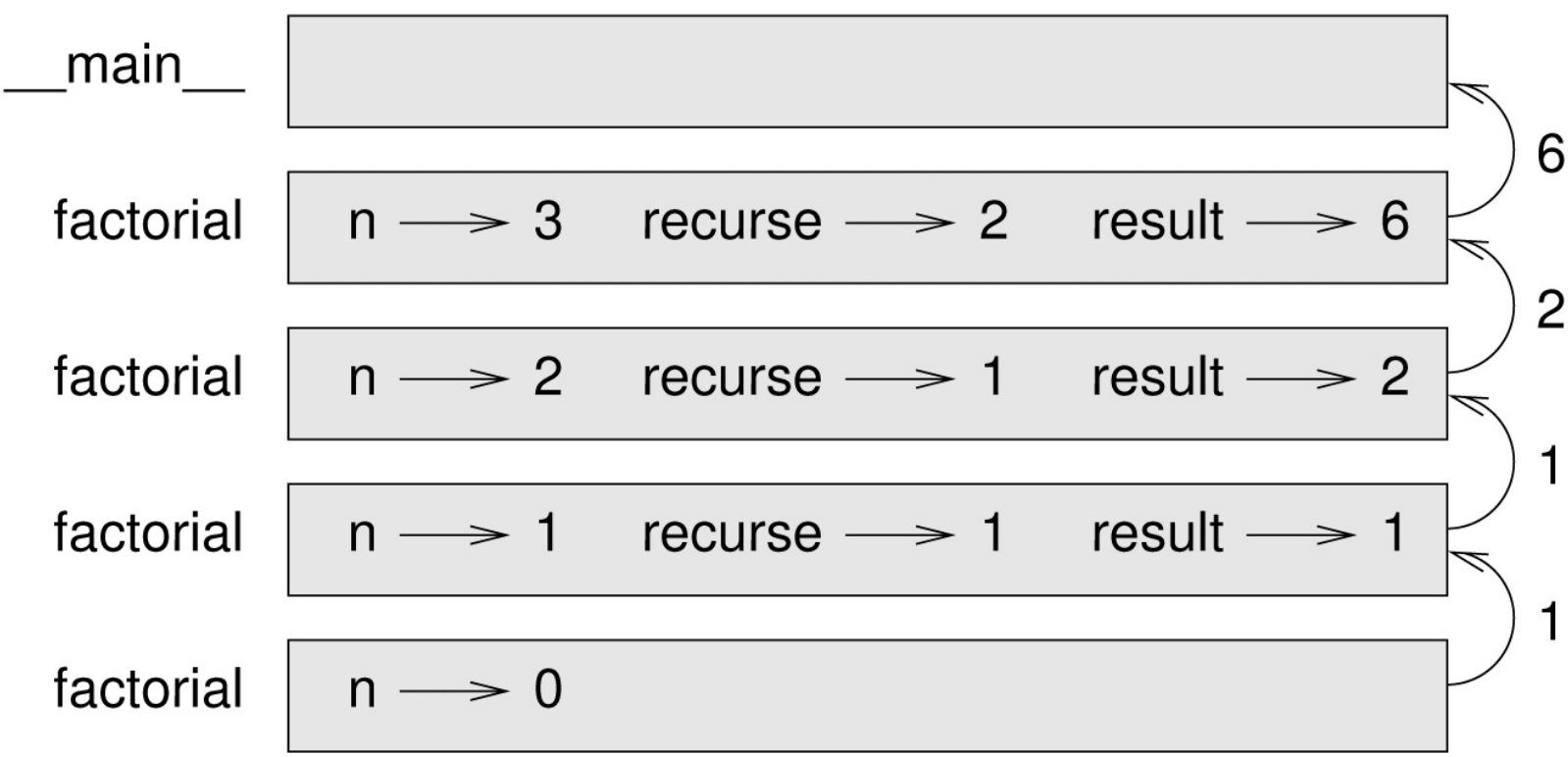
Figure 5-1. Stack diagram
