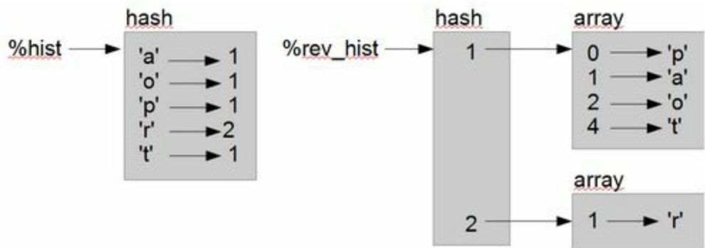
Figure 10-1. State diagram
