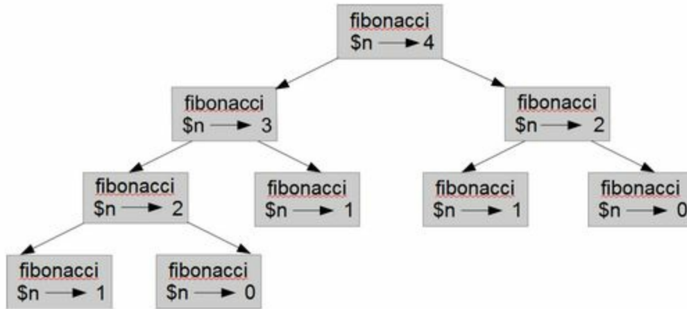
Figure 10-2. Call graph
