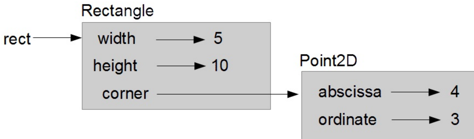
Figure 12-2. Object diagram
