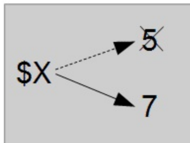
Figure 6-1. State diagram
