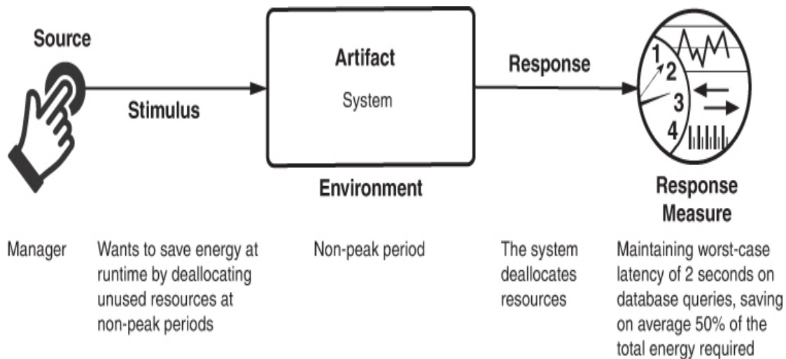
Figure 6.1 Sample energy efficiency scenario
