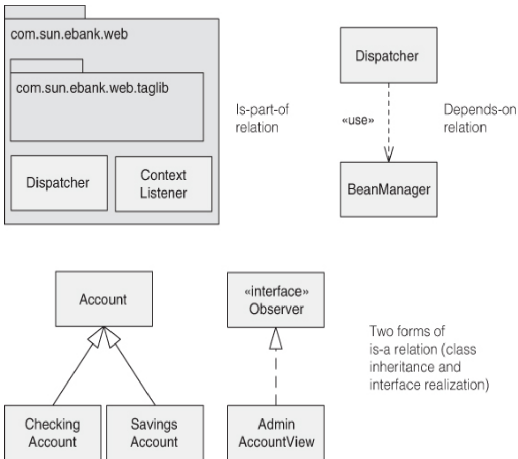
Figure 1.4 Module relations in UML
