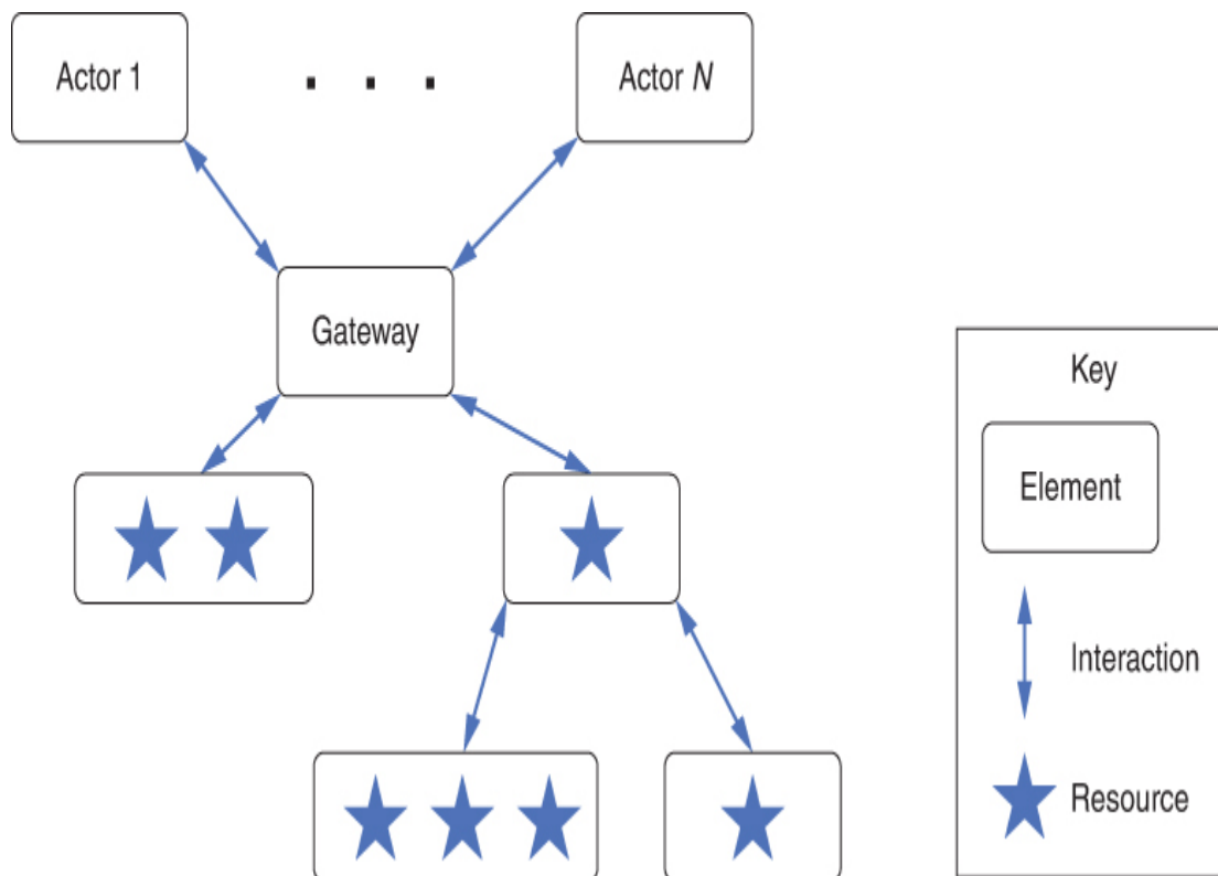
Figure 15.2 A gateway that provides access to a variety of different resources
