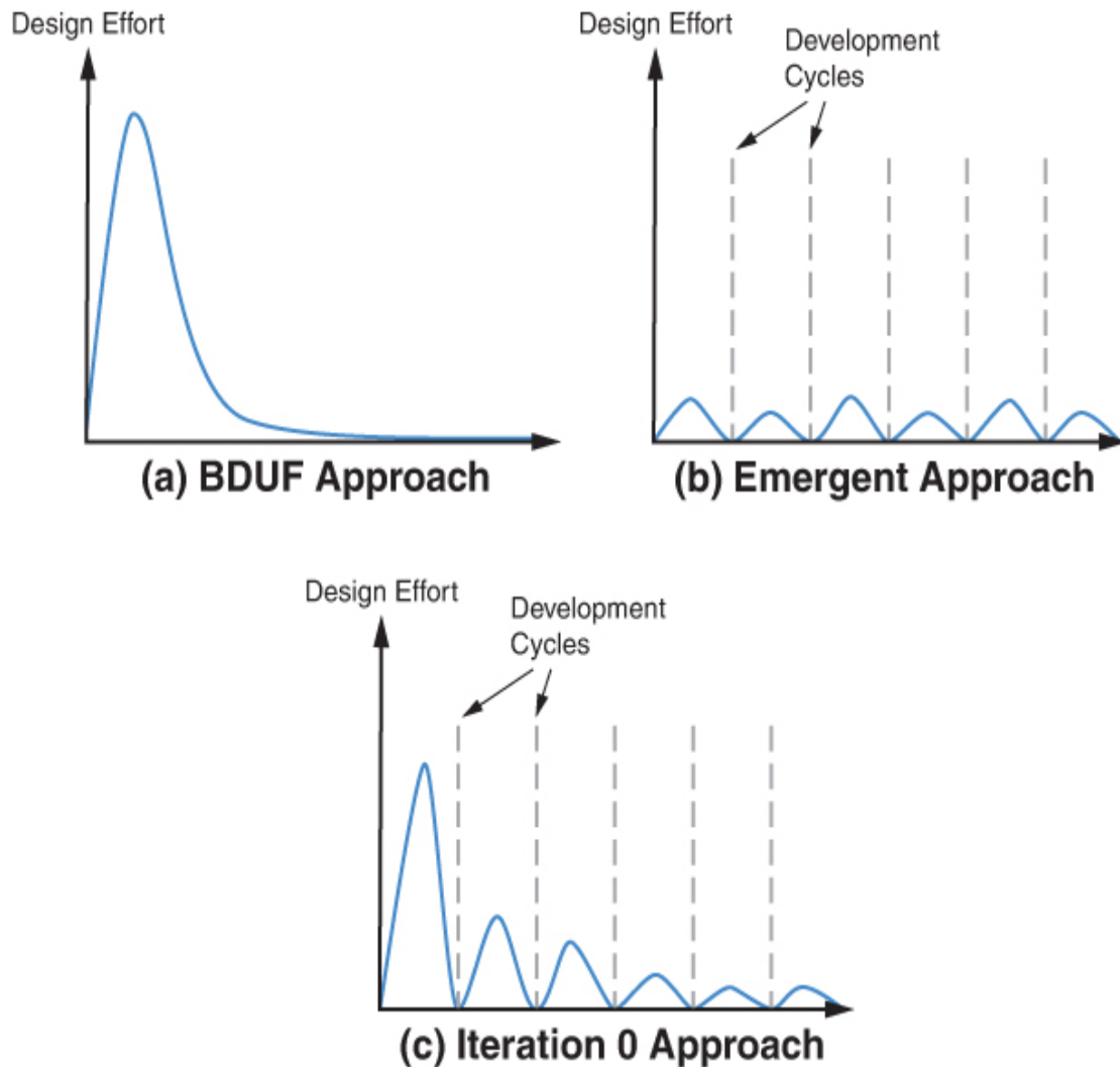
Figure 24.1 Three approaches to architectural design
