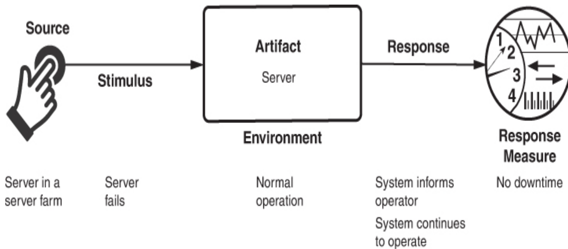
Figure 4.1 Sample concrete availability scenario
