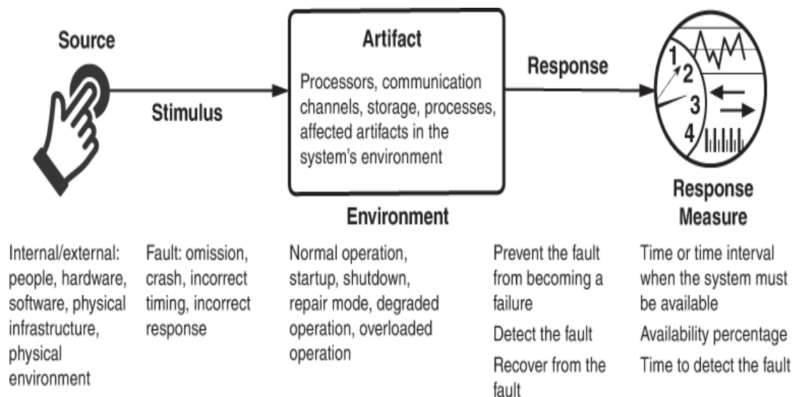
Figure 3.2 A general scenario for availability
