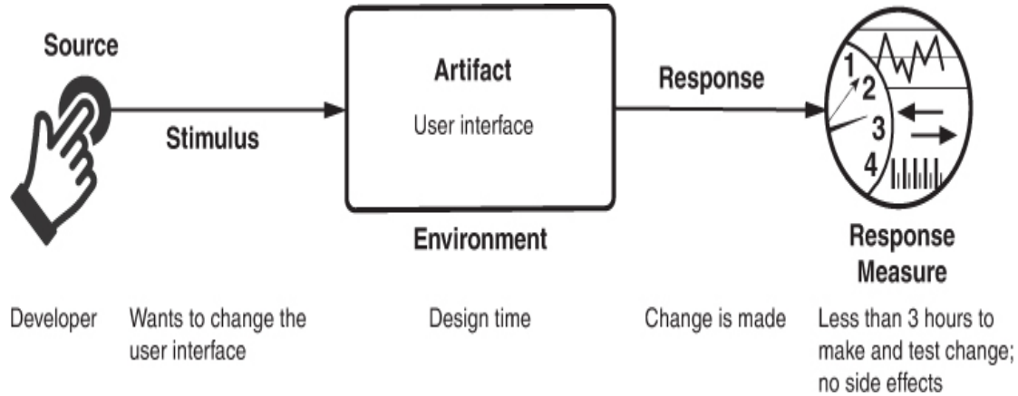
Figure 8.1 Sample concrete modifiability scenario
