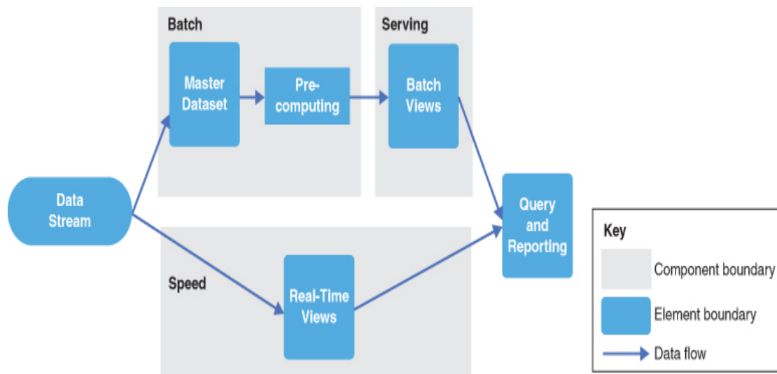
Figure 20.4 Example preliminary documentation
