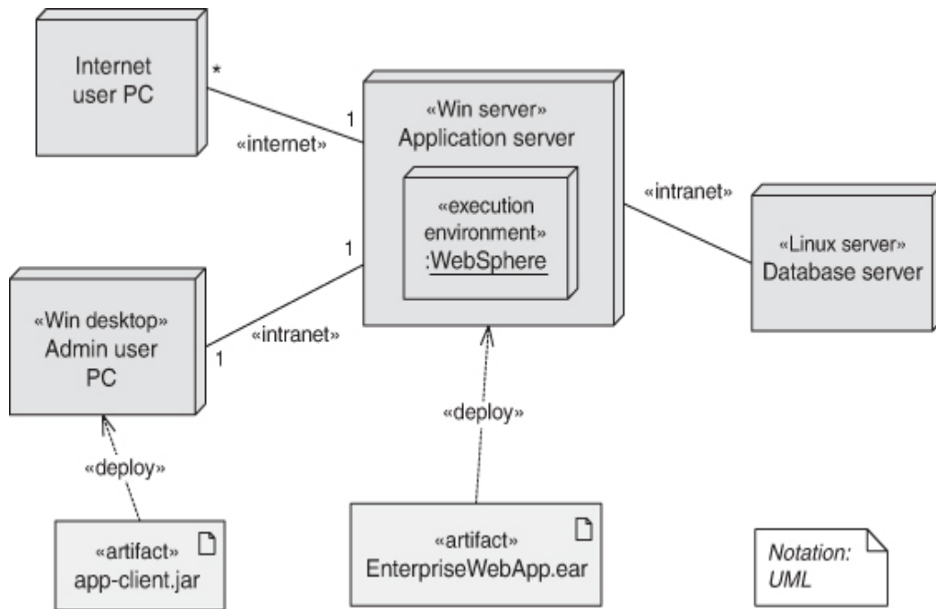
Figure 1.10 Deployment structure
