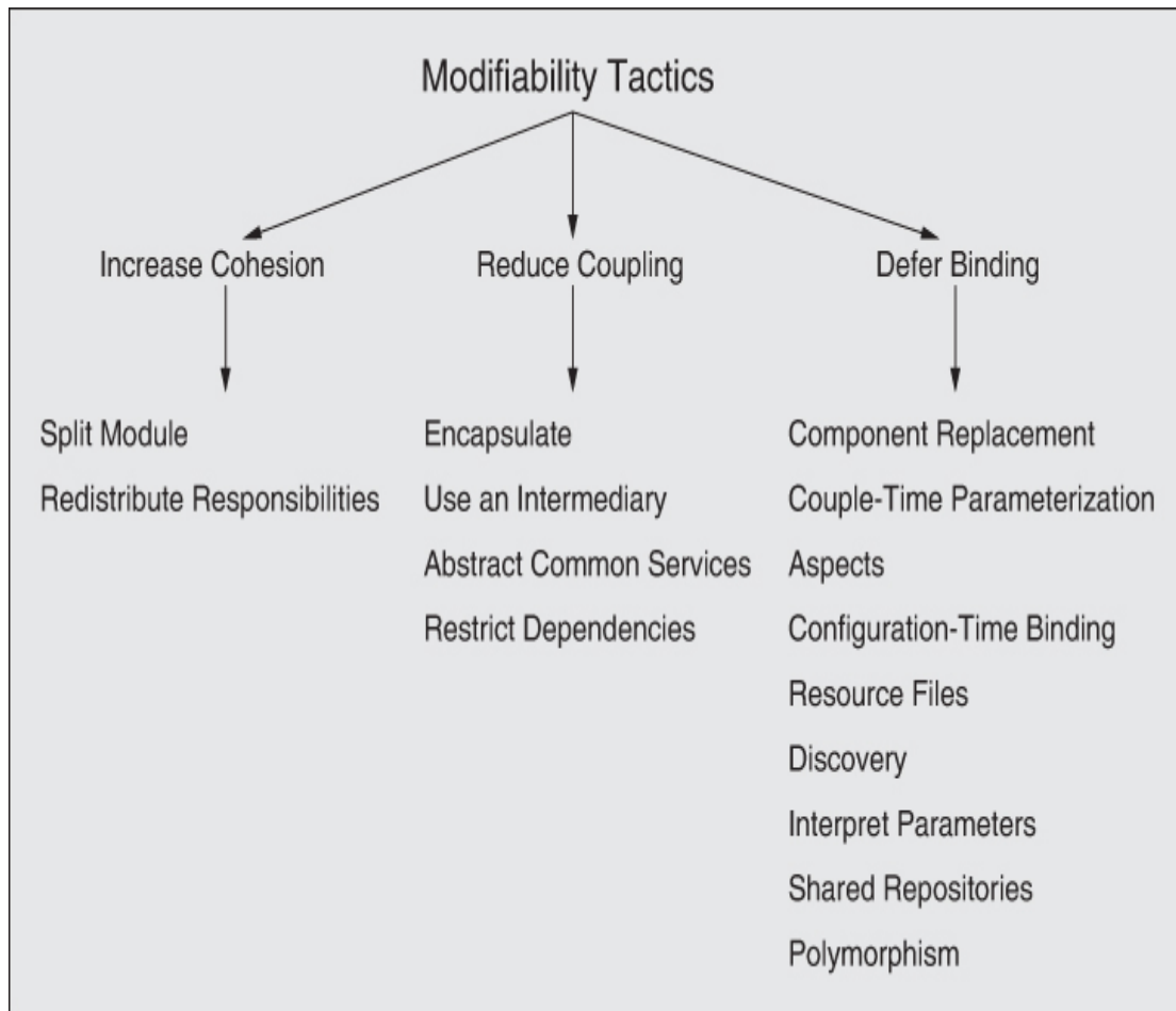
Figure 8.3 Modifiability tactics
