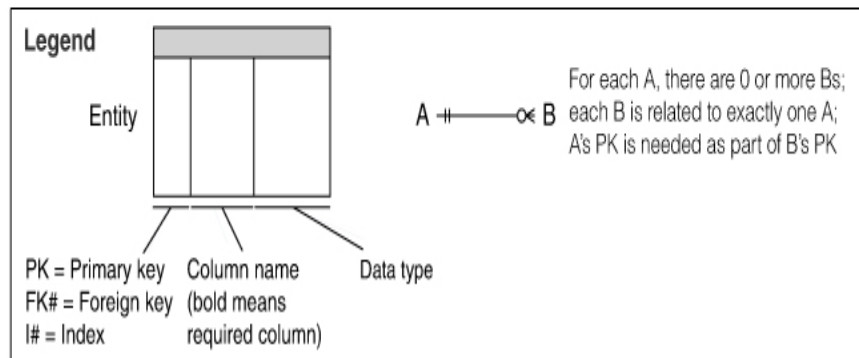
Figure 1.9 Data model
