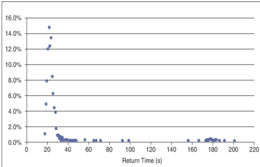
Figure 17.3 Long tail distribution of 1,000 “launch instance” requests to AWS
