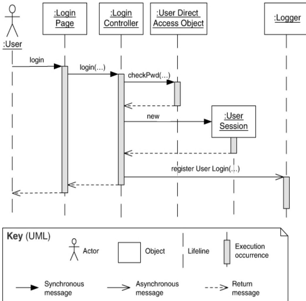
Figure 22.2 A simple example of a UML sequence diagram
