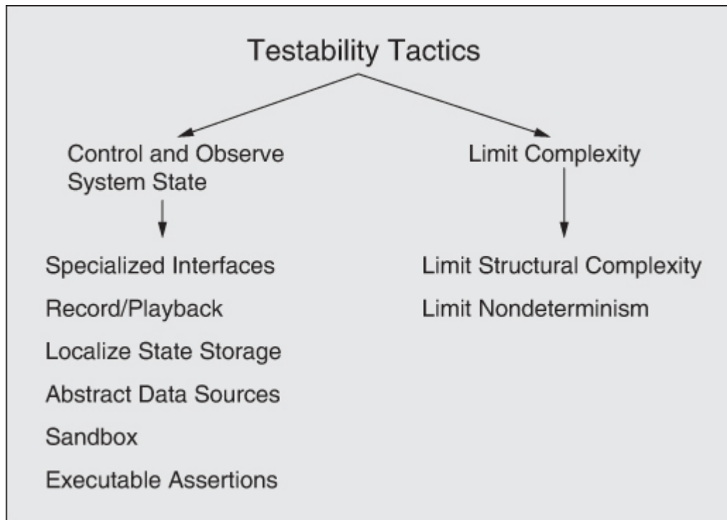
Figure 12.4 Testability tactics
