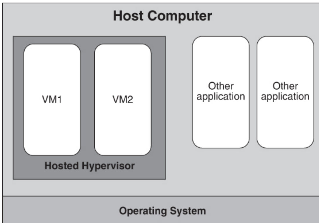
Figure 16.2 Hosted hypervisor
