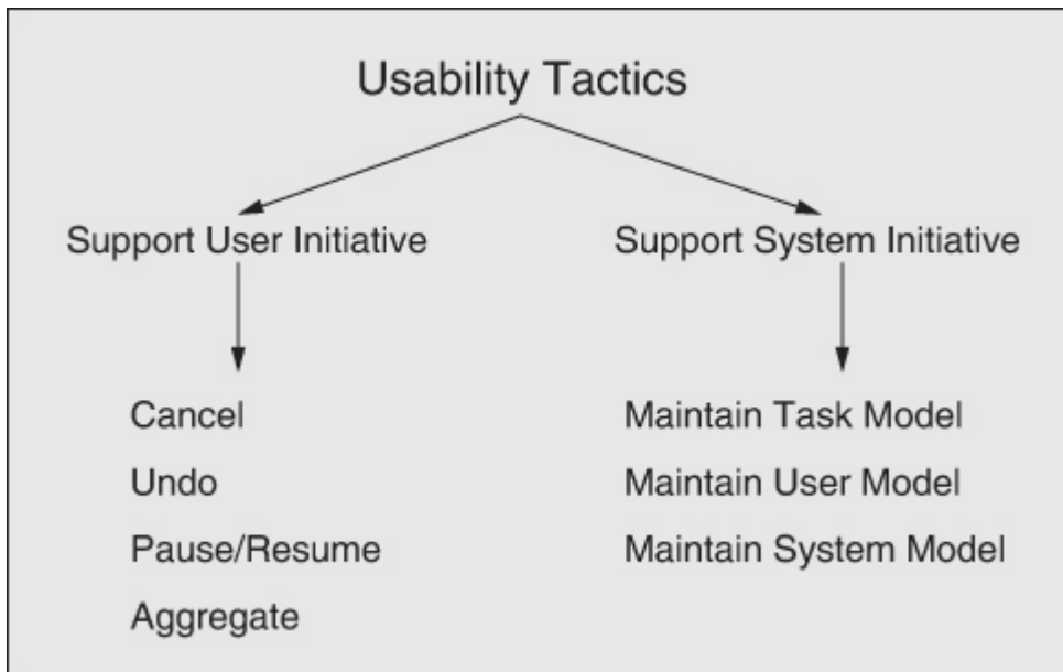
Figure 13.3 Usability tactics
