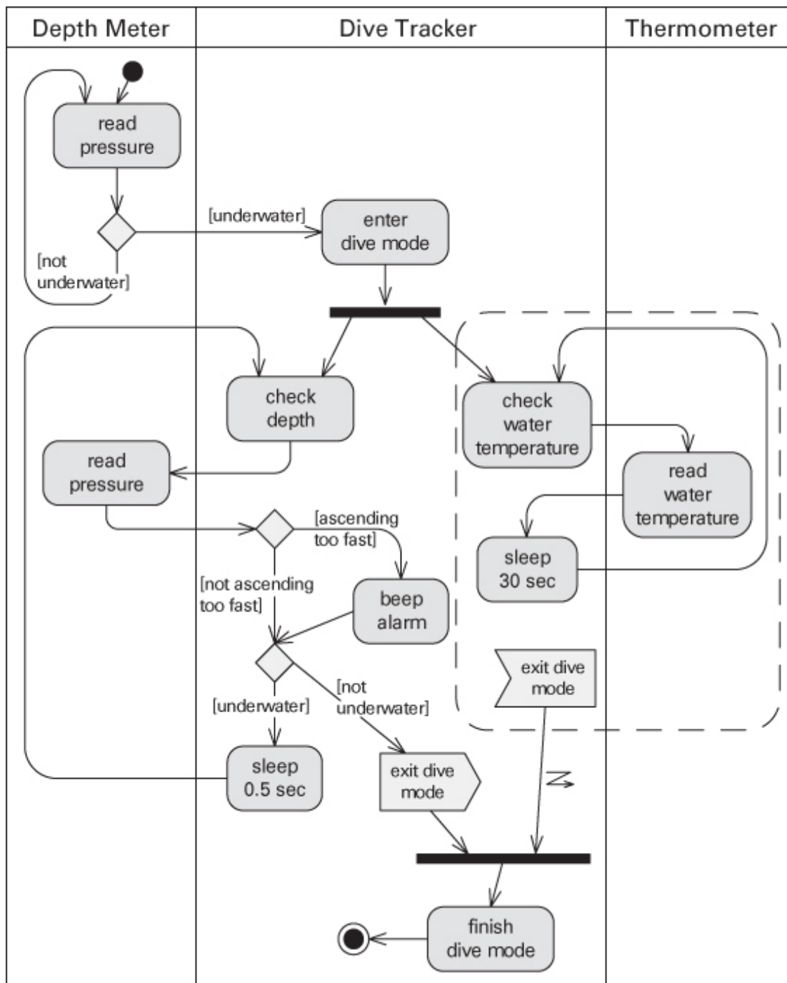
Figure 22.3 Activity diagram
