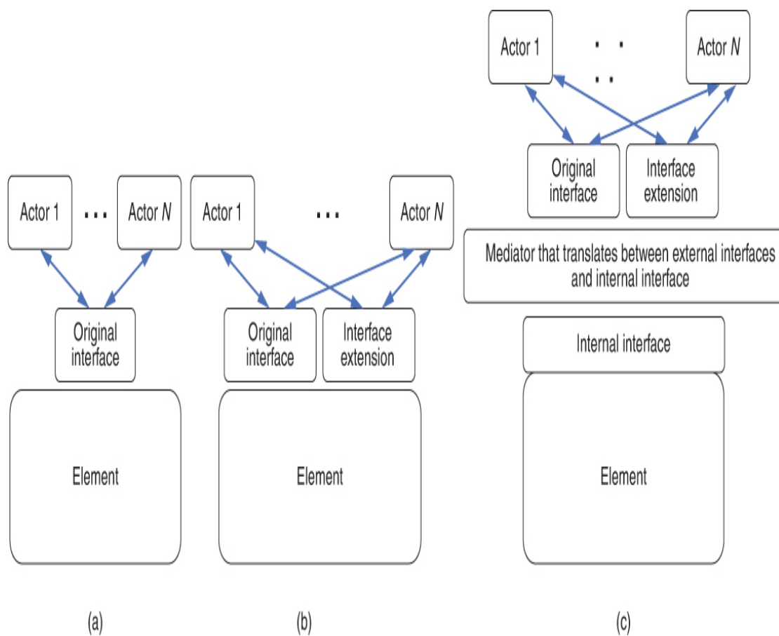
Figure 15.1 (a) The original interface. (b) Extending the interface. (c) Using an intermediary.
