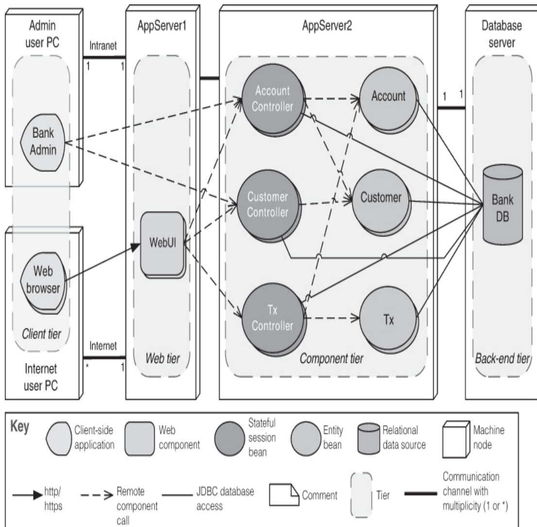
Figure 22.1 A combined view
