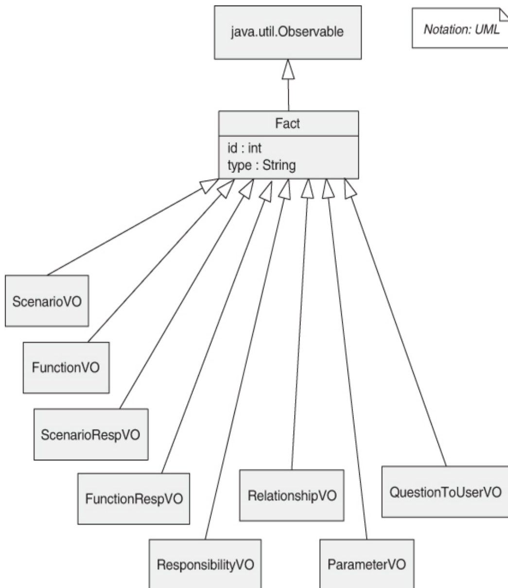
Figure 1.8 Generalization structure
