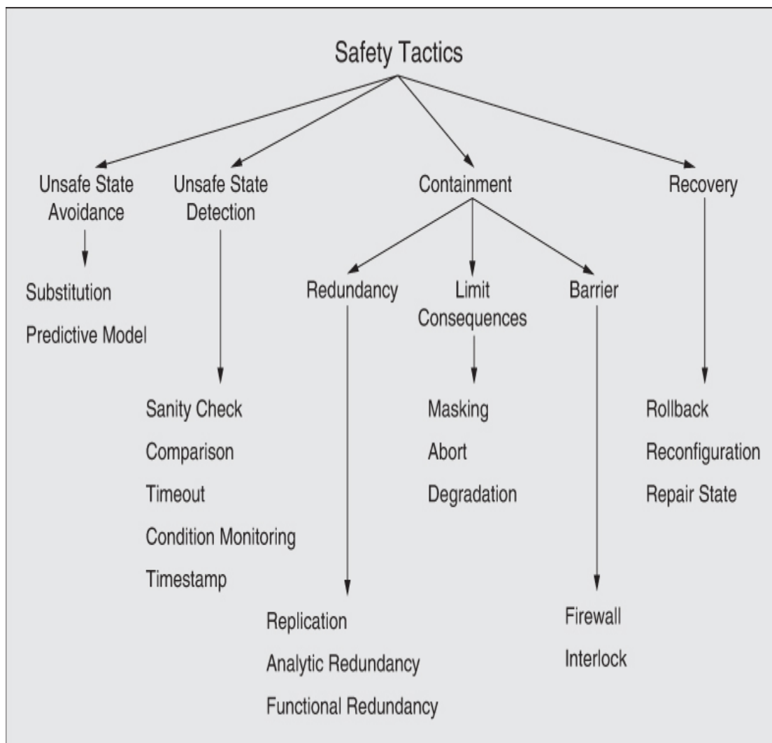
Figure 10.3 Safety tactics
