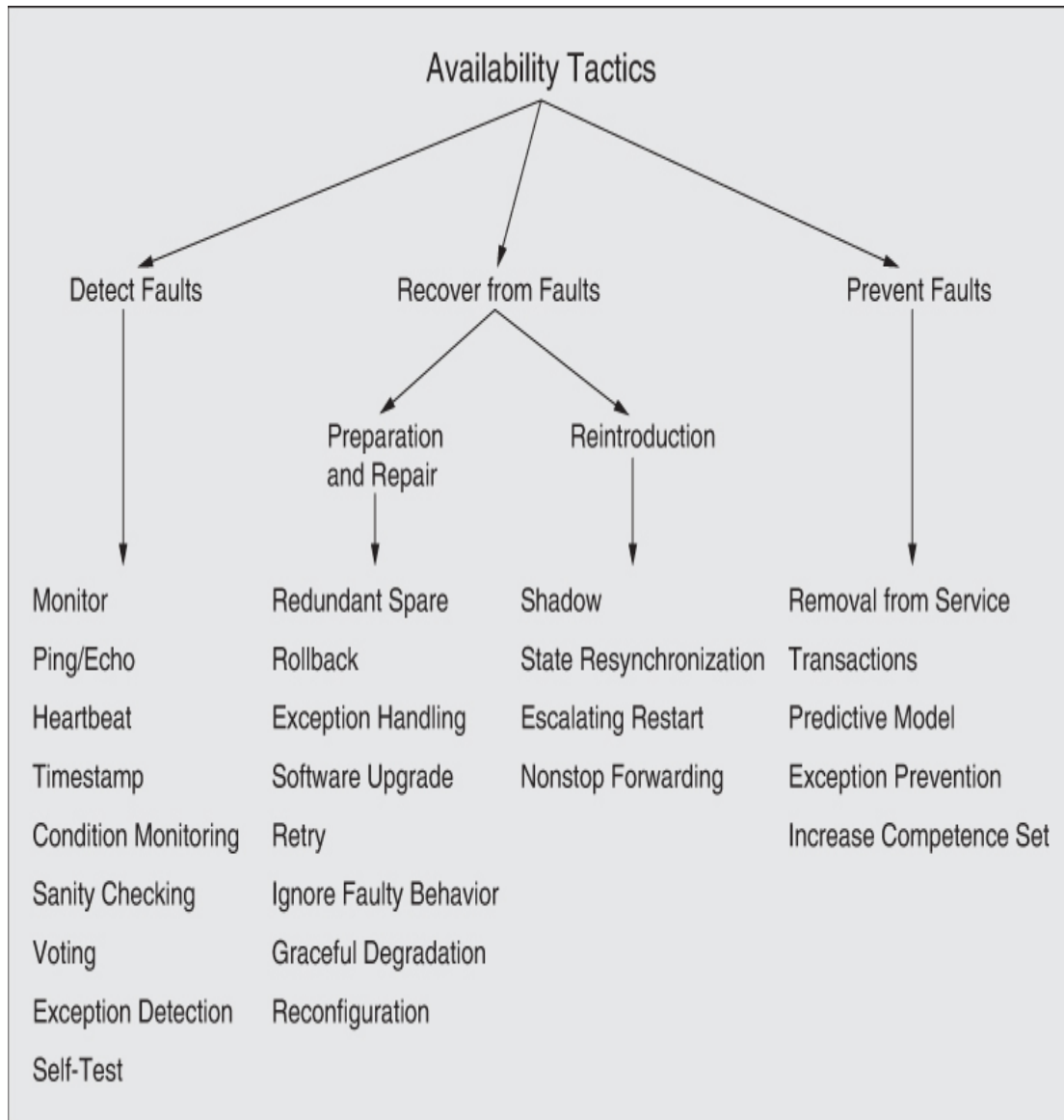
Figure 4.3 Availability tactics
