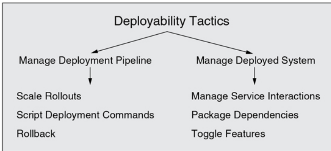
Figure 5.3 Deployability tactics
