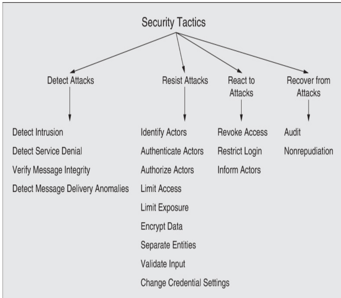
Figure 11.3 Security tactics
