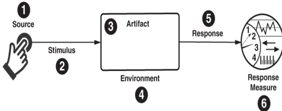
Figure 3.1 The parts of a quality attribute scenario
