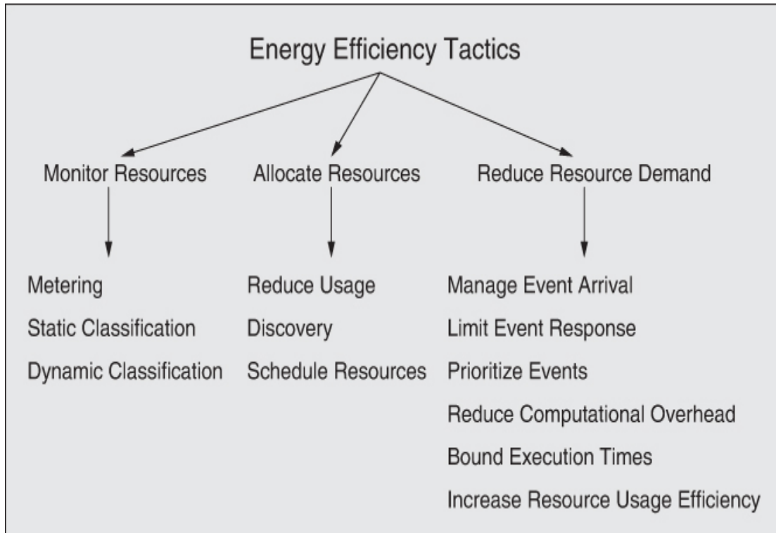
Figure 6.3 Energy efficiency tactics
