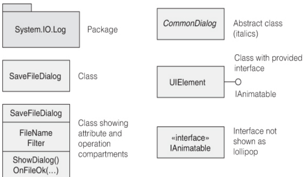
Figure 1.3 Module elements in UML
