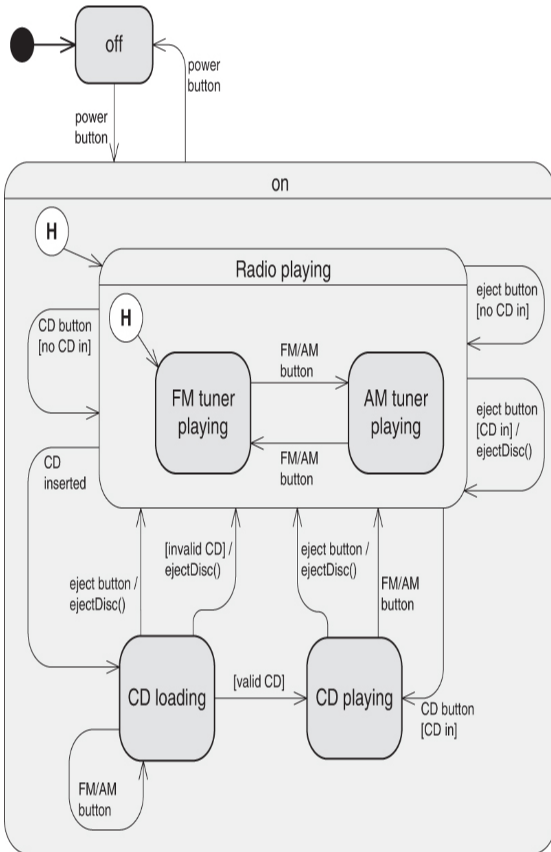
Figure 22.4 UML state machine diagram for a car stereo system
