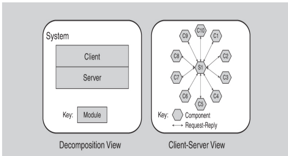
Figure 1.11 Two views of a client-server system
