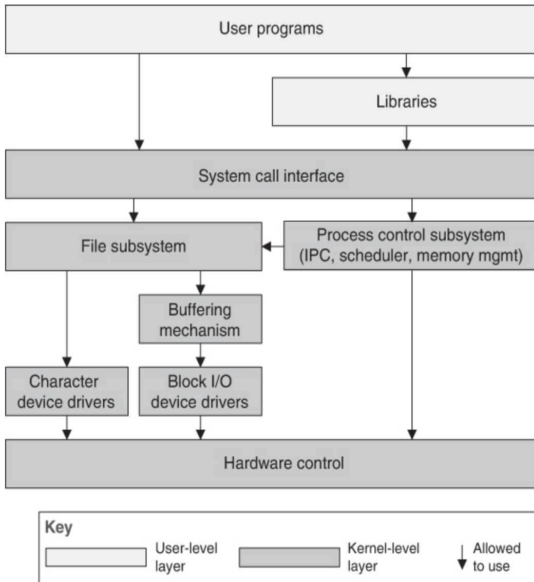
Figure 1.7 Layer structure
