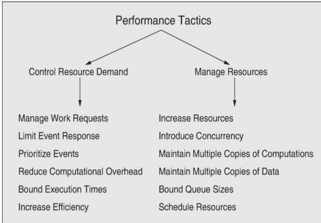
Figure 9.3 Performance tactics
