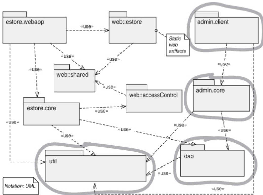
Figure 1.6 Uses structure
