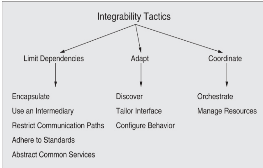
Figure 7.3 Integrability tactics
