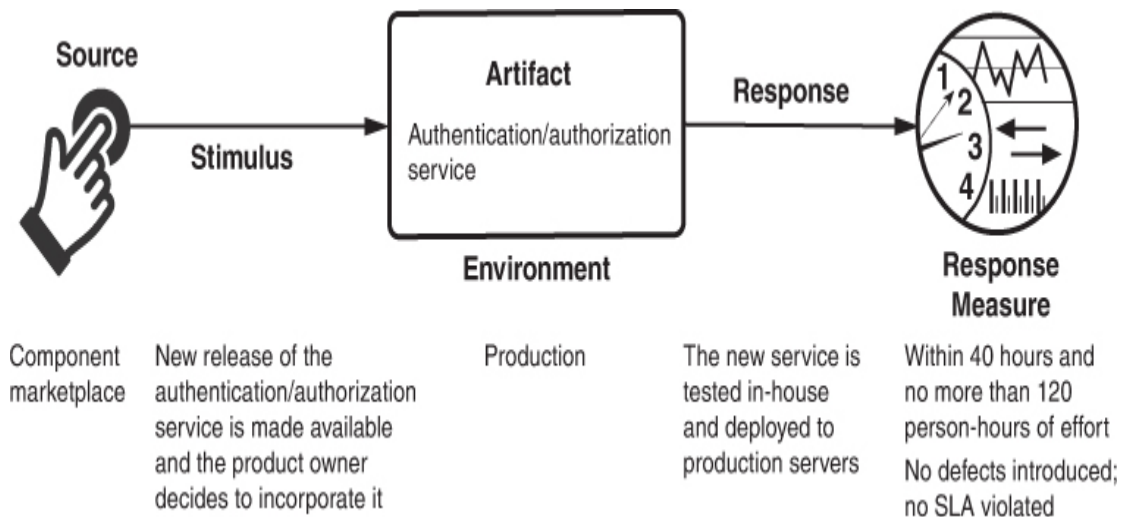
Figure 5.1 Sample concrete deployability scenario
