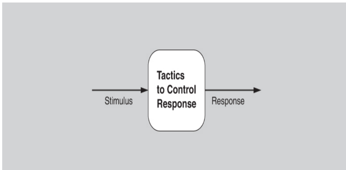
Figure 3.3 Tactics are intended to control responses to stimuli.
