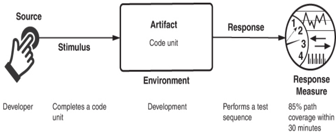
Figure 12.2 Sample testability scenario
