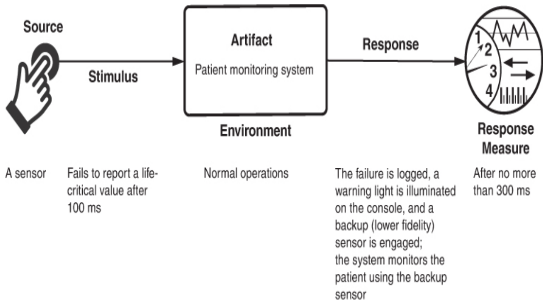
Figure 10.1 Sample concrete safety scenario
