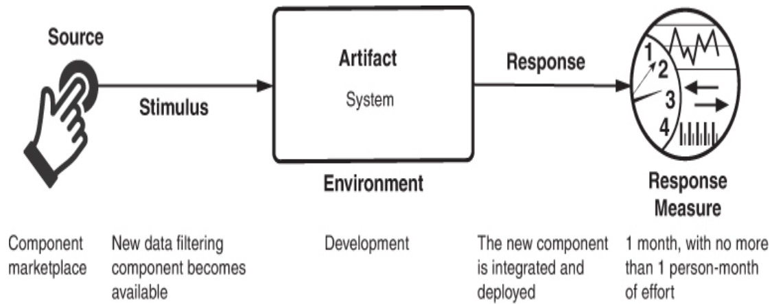
Figure 7.1 Sample integrability scenario
