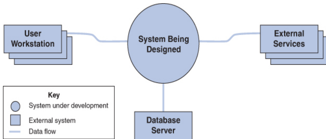
Figure 20.2 Example of a system context diagram
