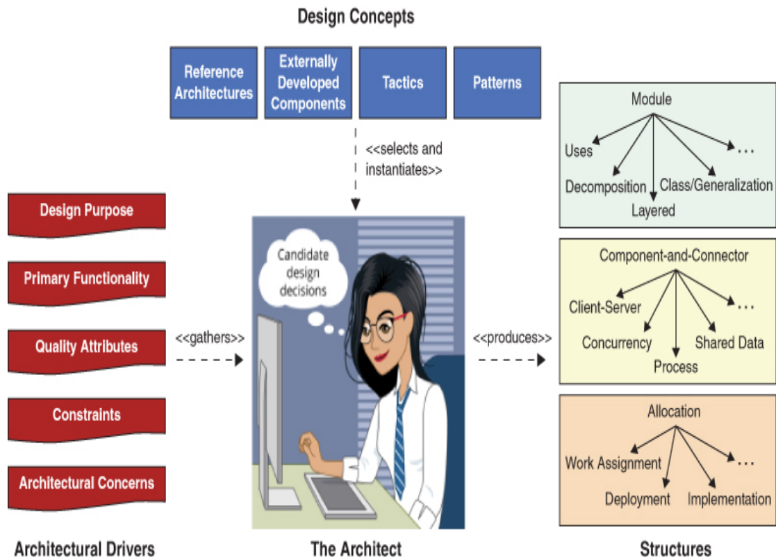
Figure 20.1 Overview of the architecture design activity
