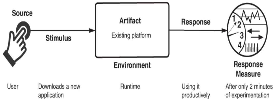
Figure 13.1 Sample usability scenario
