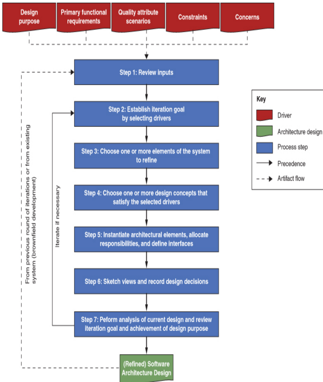
Figure 20.3 Steps and artifacts of ADD
