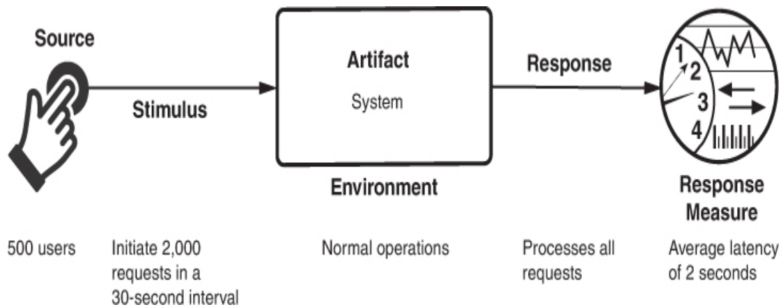
Figure 9.1 Sample performance scenario
