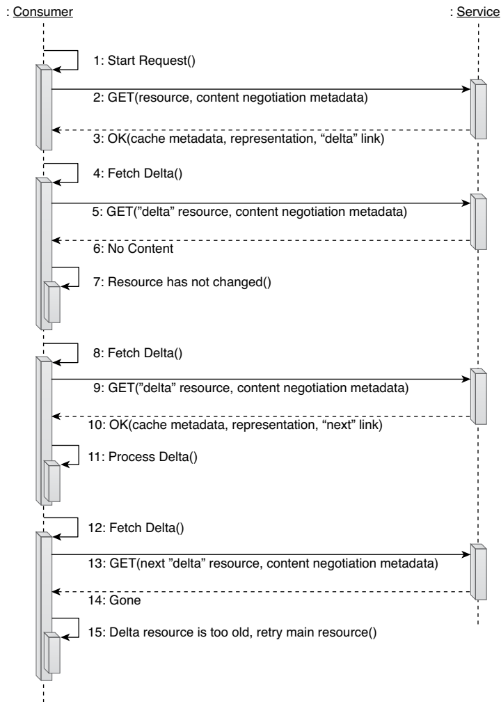
Figure 9.14 An example of the message interaction encompassed by the Delta complex method.
