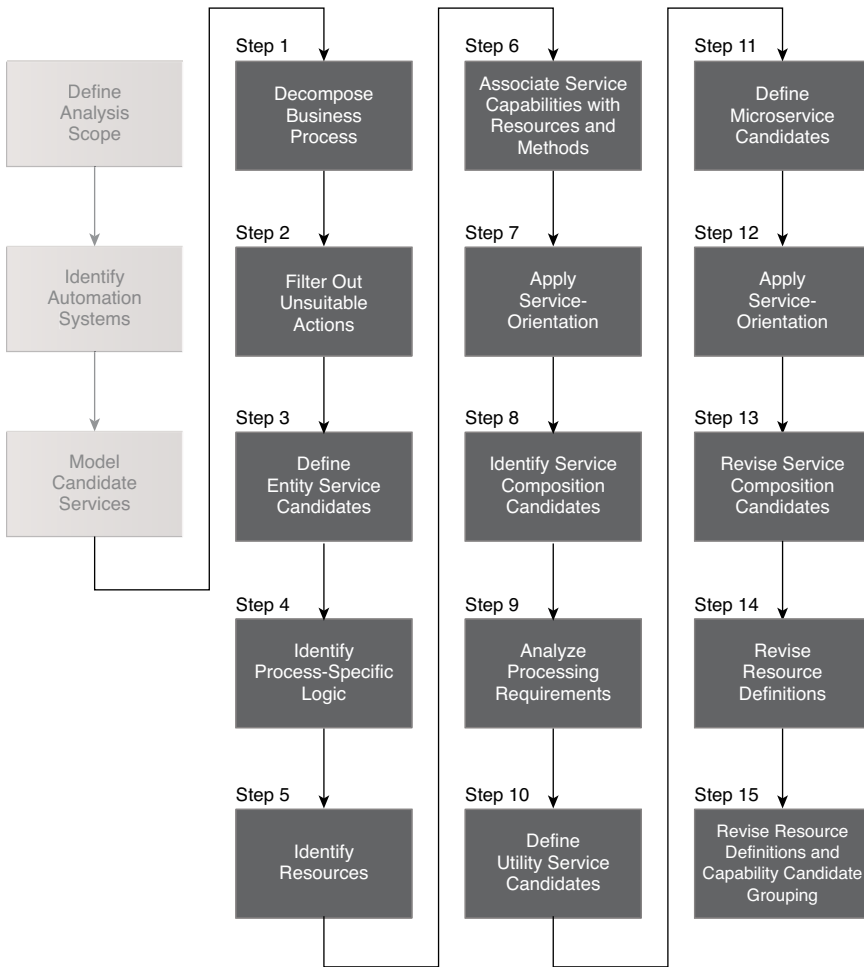
Figure 7.1 A sample service modeling process for REST services.
