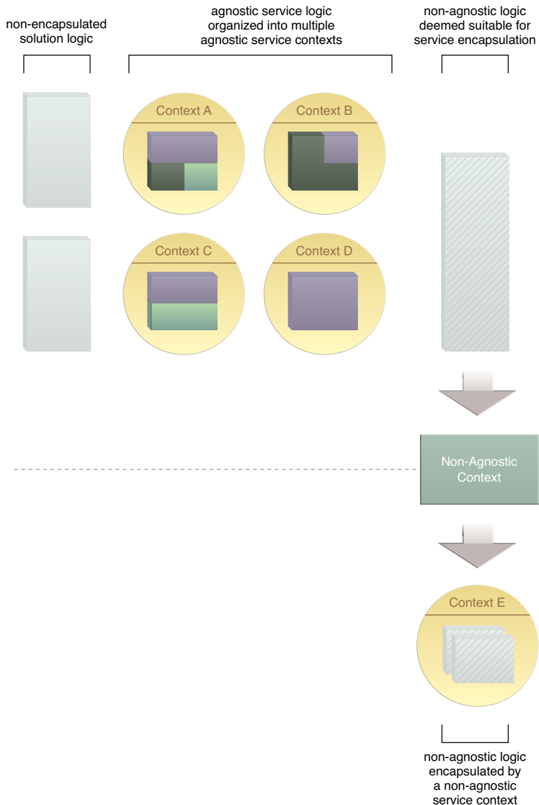
Figure 5.9 By revisiting the decomposition process, the remaining service logic can now be categorized as non-agnostic.
